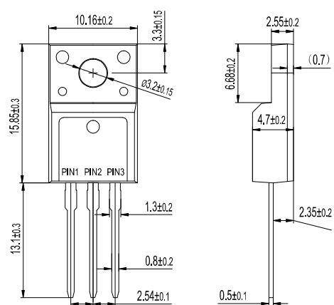
ITO-220AB HER10XXFCT
