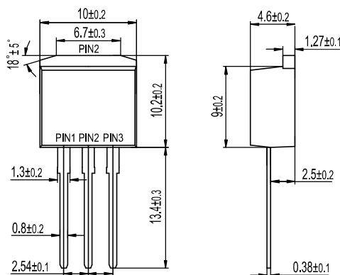
TO-262AB HER10XXWCT
