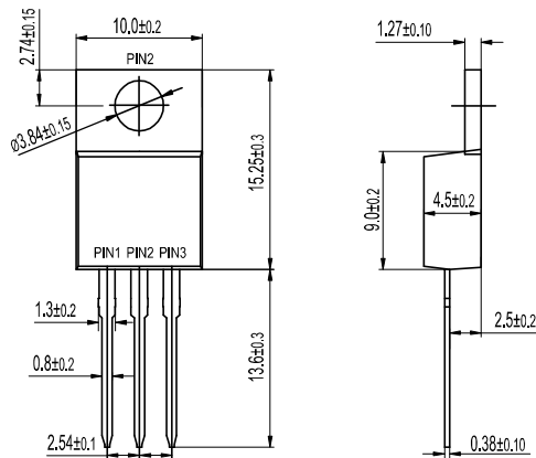
TO-220AB HER10XXCT
